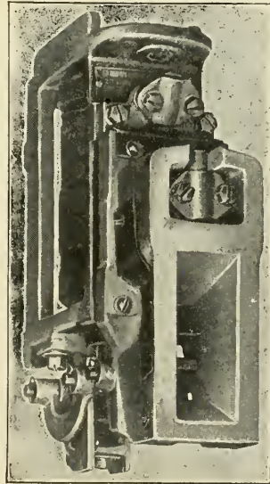
Fig. 59. Sprague-General Electric Contactor
